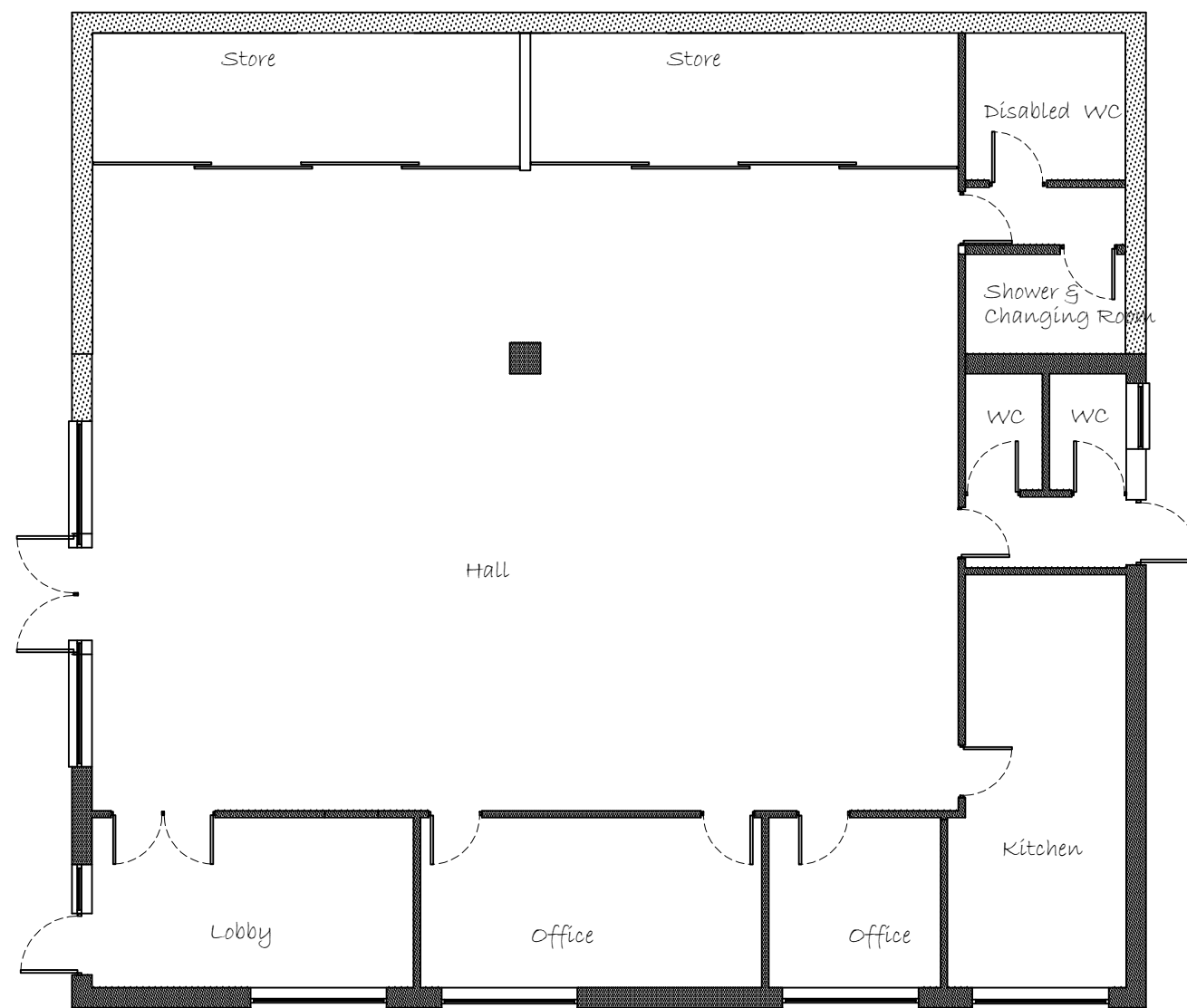
Floor Plan Layout
